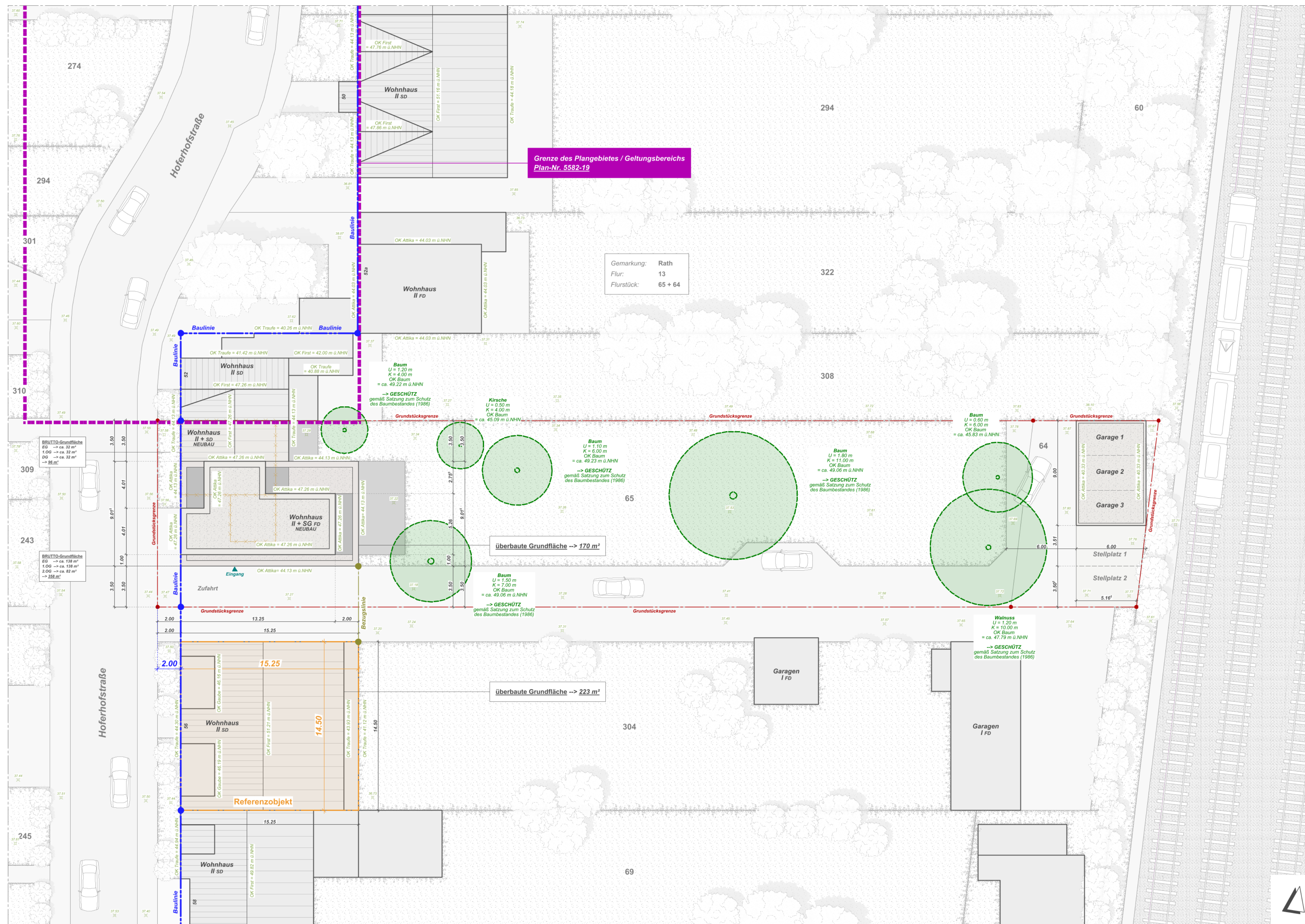
Lageplan | M 1: 200
