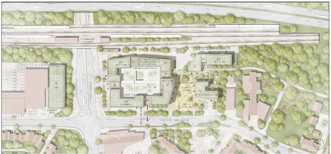
Lageplan - o.M.
